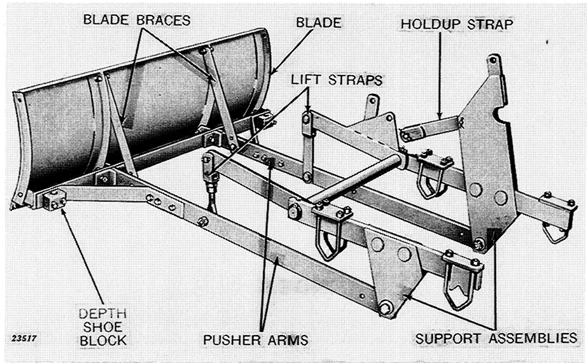
MC60 Bulldozer—For John Deere Model "MC" Tractor and "40" Crawler Tractor with Three- and Four-Roller Track
