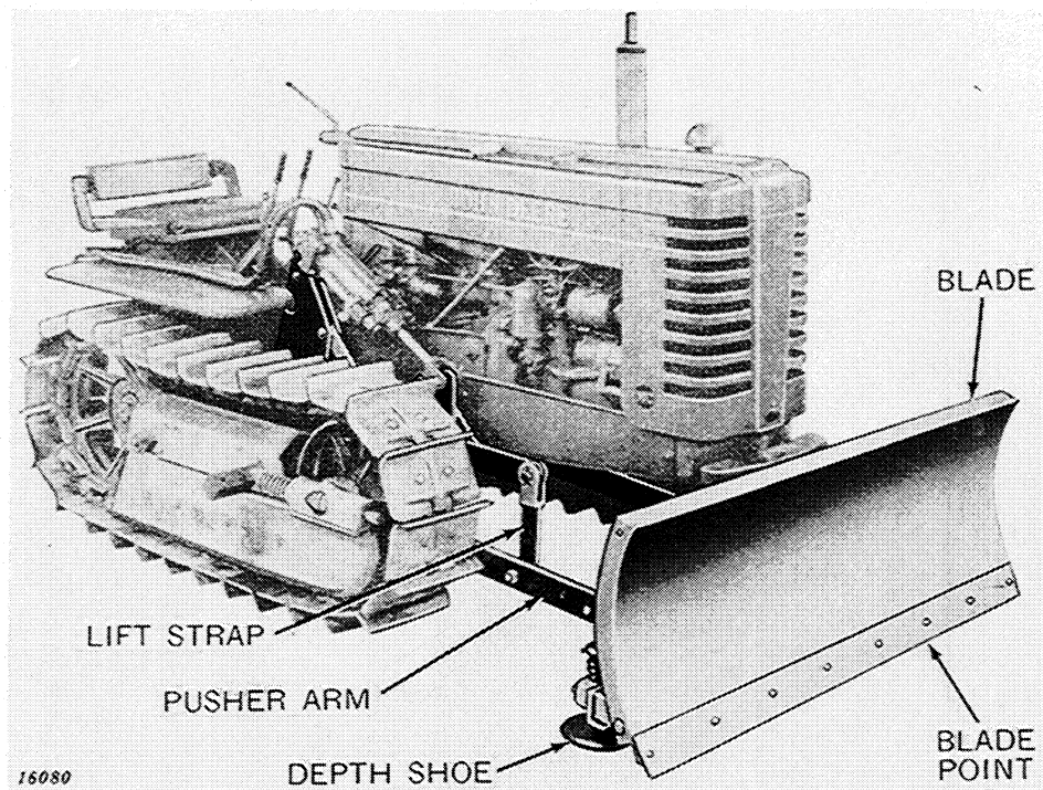
John Deere Model "MC" Tractor with MC60 Bulldozer
