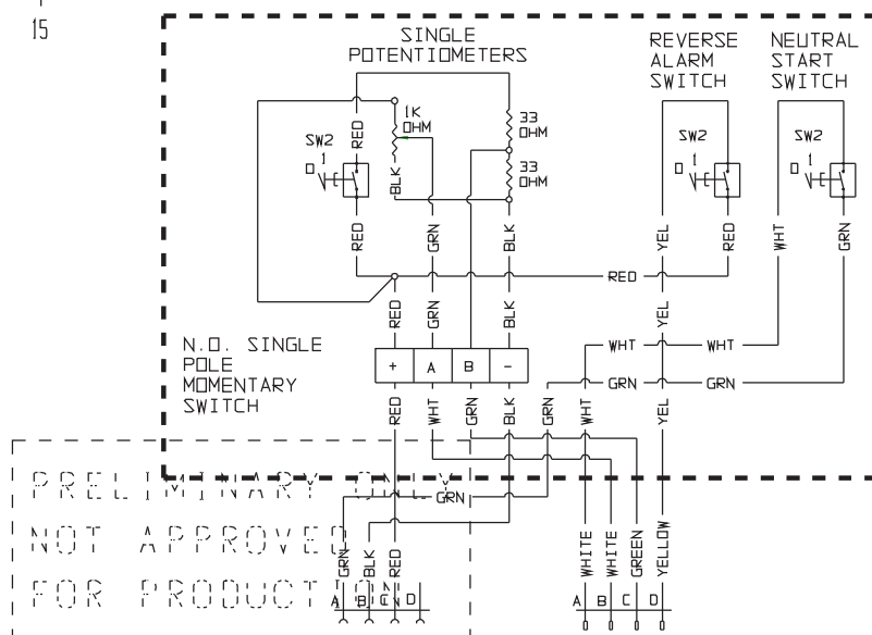
GROUND DRIVE MXX275B CONTROL HANDLE WIRING DIAGRAM
